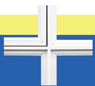
Bevelled Exterior Frame & Unbalanced Sash
